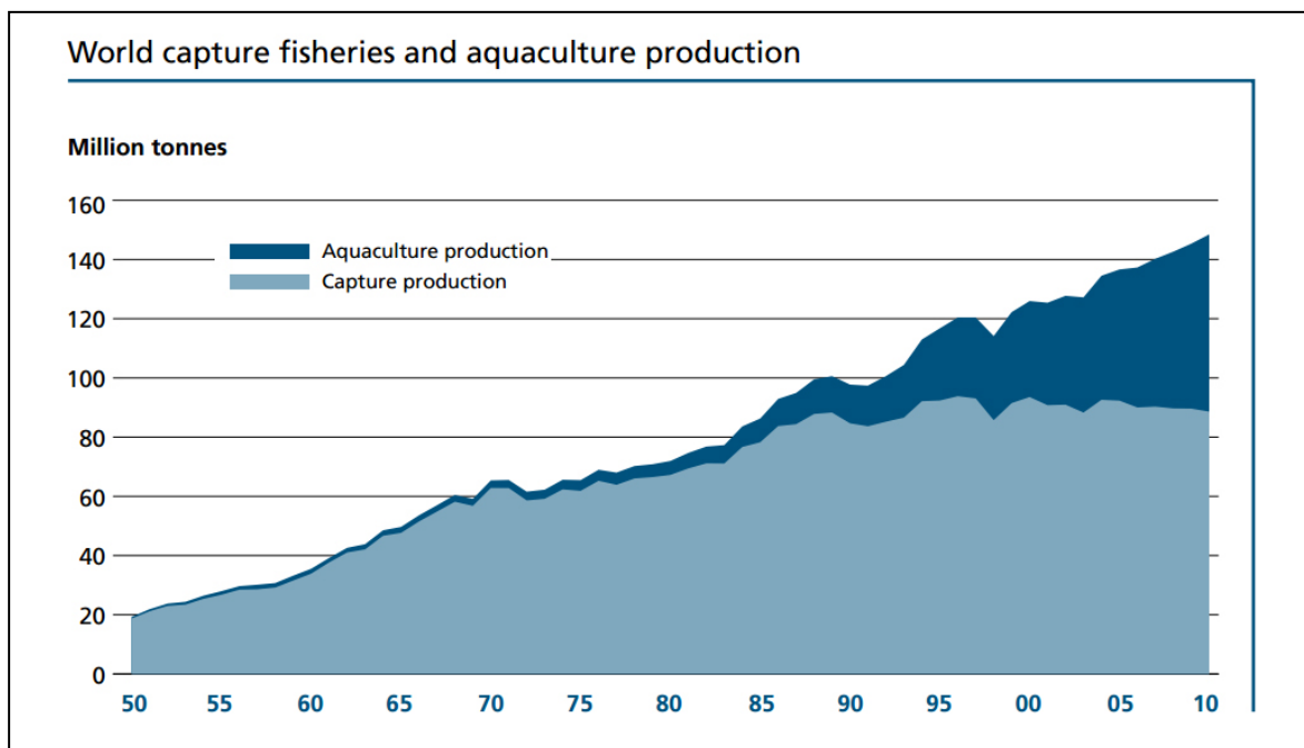
Figure D5.3. Comparison of fishery production and aquaculture, 1950-2010
